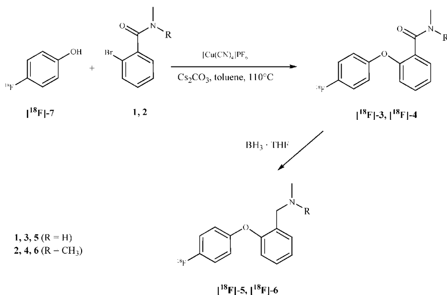
Scheme 3. Synthesis of n.c.a. 2-(4-[ 18 F]fluorophenoxy)-benzylamines [ 18 F]-5 and [ 18 F]-6 via an Ullmann ether synthesis starting with n.c.a. 4-[ 18 F]fluorophenol and corresponding 2-bromobenzamides 1 and 2
